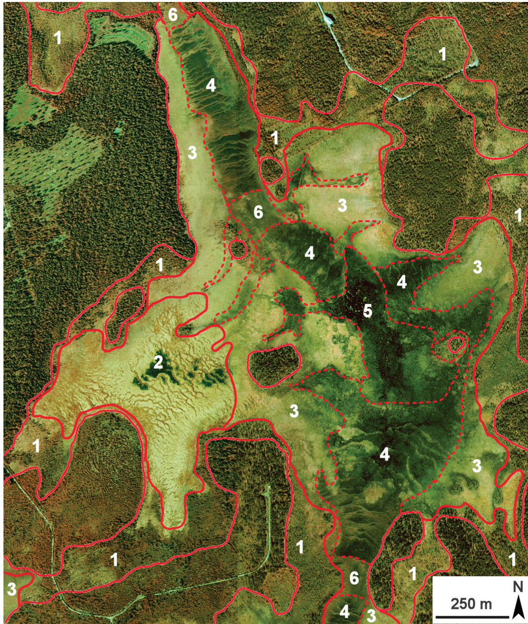
Fig. 2. The CFMT applied for the Hoikkasuo mire (65° 42' N, 25° 1' E, c. 70 m a.s.l., see Fig. 1), an aapa mire system with a raised bog. The mire system has marginal areas (1) around mire massifs, a patterned eccentric bog massif (2) and a lawn-flark aapa mire massif in the N-S direction. In the aapa mire massif, there are peripheral lobes (3) interrupted by soaks, string flark fens (4), stringless central flark fens (5) and outlet fens (6). Unit 3 (with soaks) forms the peripheral part and units 4–6 the central basin of the aapa mire massif. The patterns have been drawn on the basis of aerial photograph interpretation.
