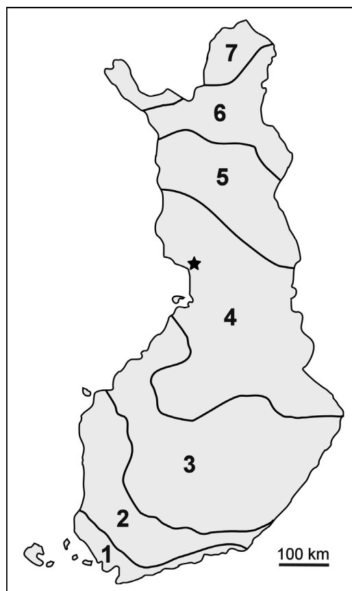
Fig. 1. Mire zones of Finland and the location of the Hoikkasuo mire system presented in Figs. 2 and 3. Mire zones according to Ruuhijärvi & Hosiaislouma (1988): 1: plateau bogs, 2: concentric bogs, 3: eccentric bogs, 4: southern aapa mires, 5: main aapa mire zone, 6: northern aapa mires, 7: palsa mires.
